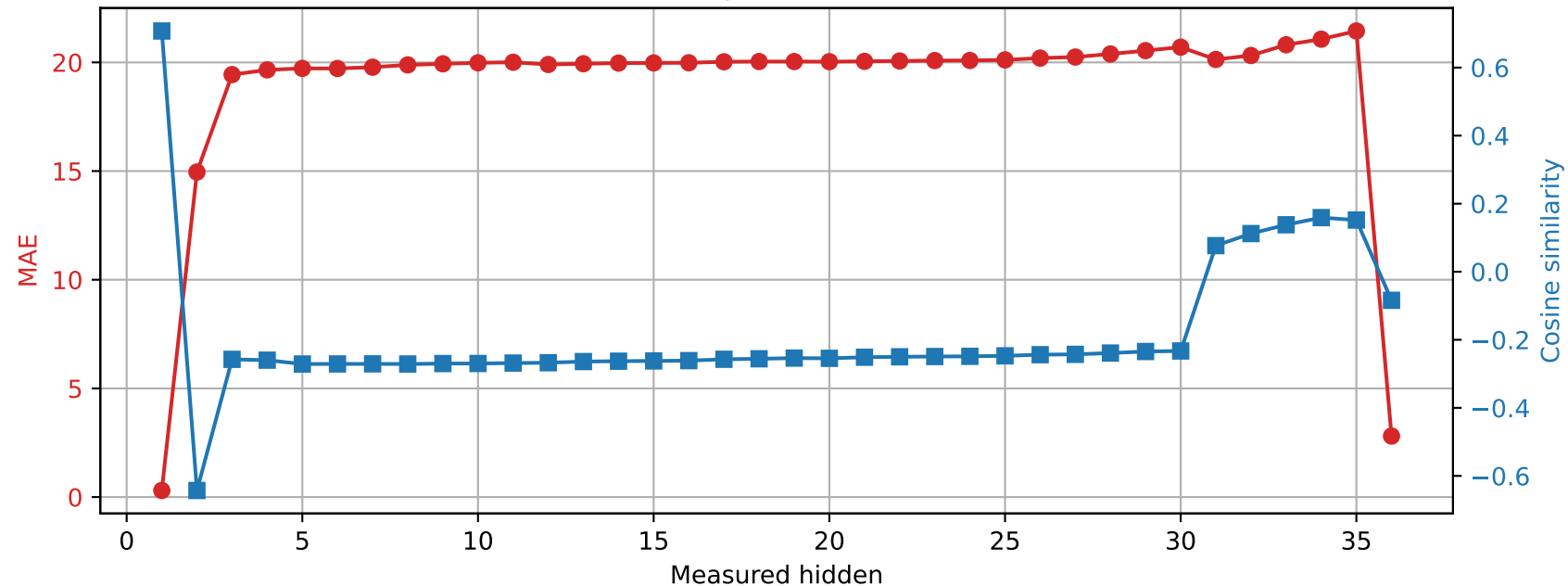
Qwen2.5-3B | Prompt 3 Spared layer 11 | Unquantized vs hybrid
