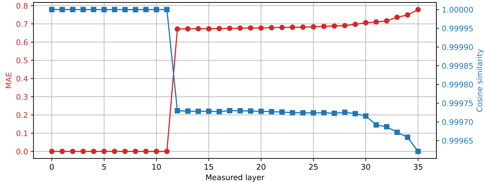
Qwen2.5-3B | Prompt 3 Spared layer 11 | Hybrid vs quantized
