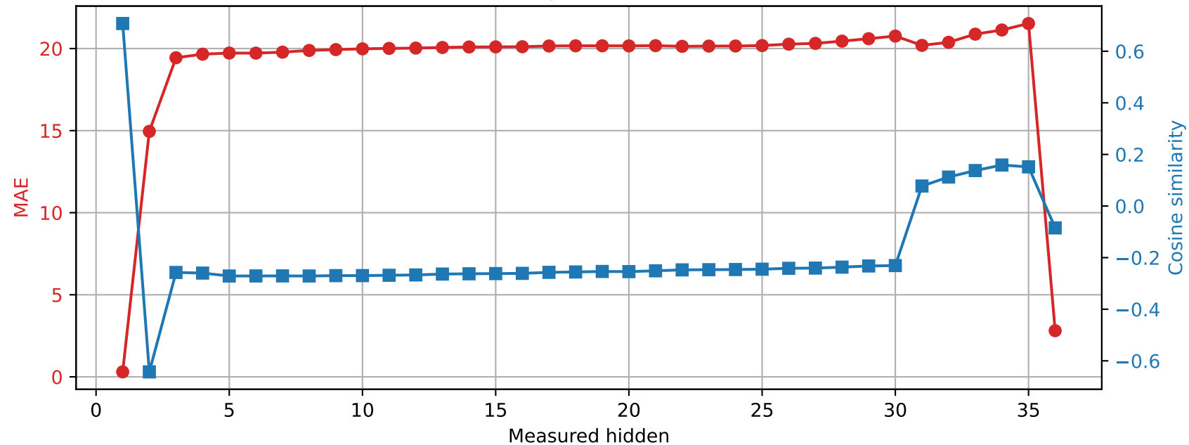
Qwen2.5-3B | Prompt 3 Spared layer 21 | Unquantized vs hybrid
