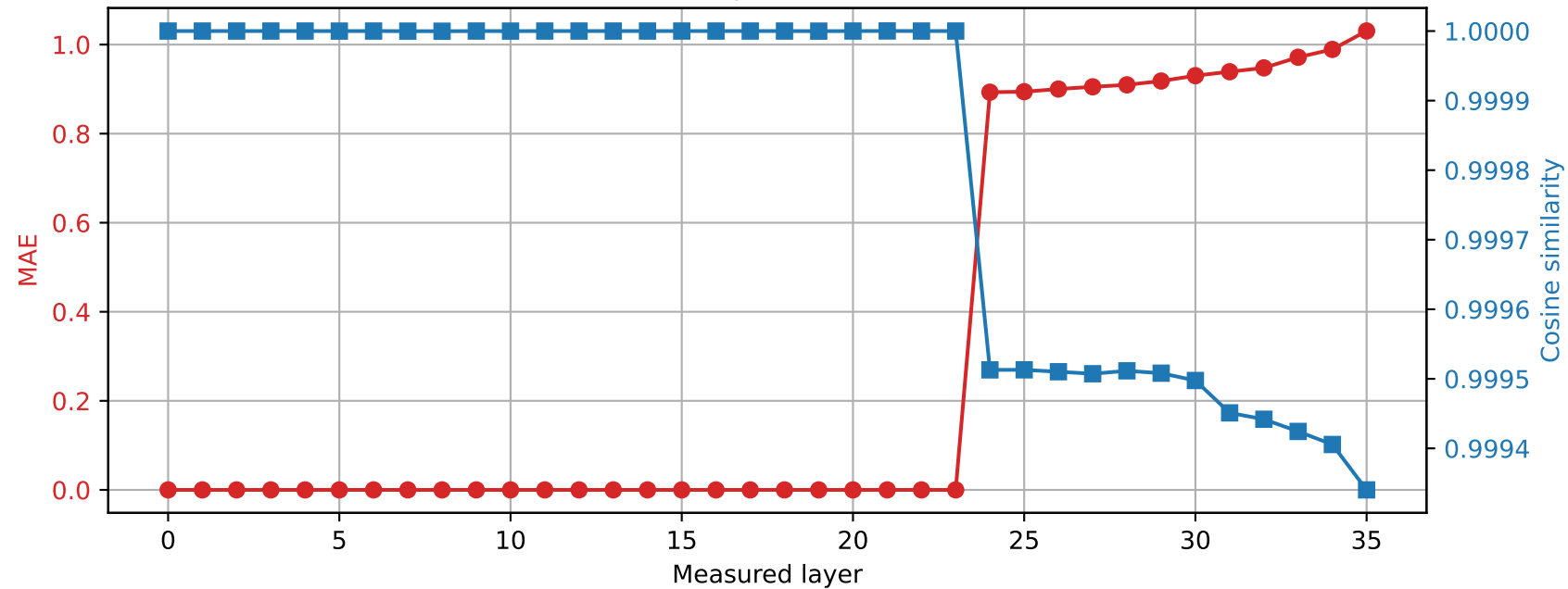
Qwen2.5-3B | Prompt 3 Spared layer 23 | Hybrid vs quantized
