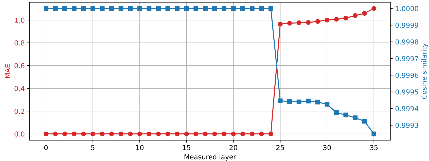
Qwen2.5-3B | Prompt 3 Spared layer 24 | Hybrid vs quantized
