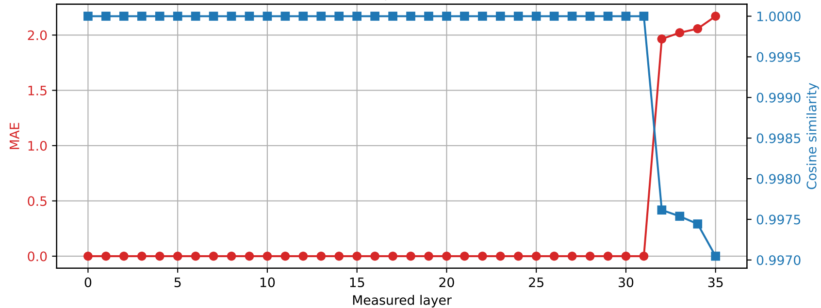
Qwen2.5-3B | Prompt 3 Spared layer 31 | Hybrid vs quantized
