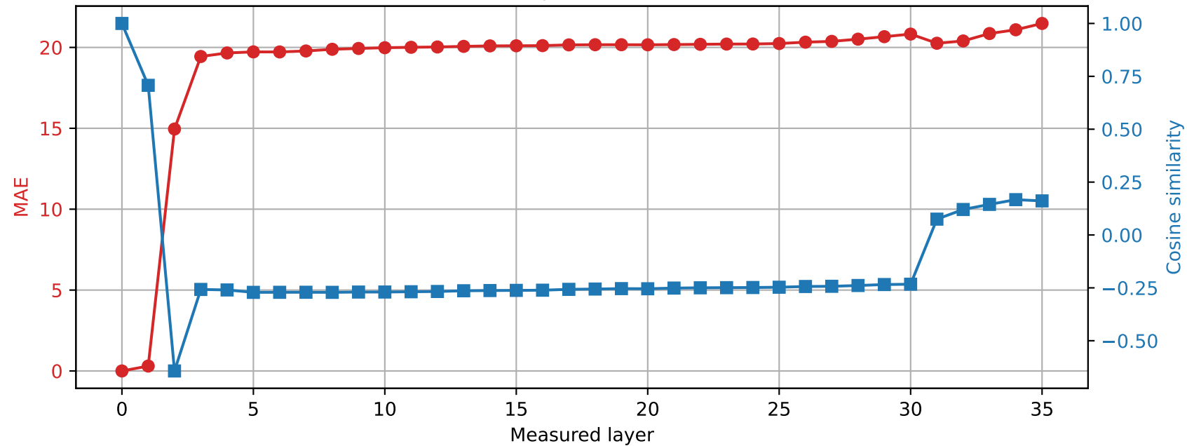
Qwen2.5-3B | Prompt 3 Spared layer 31 | Hybrid vs unquantized
