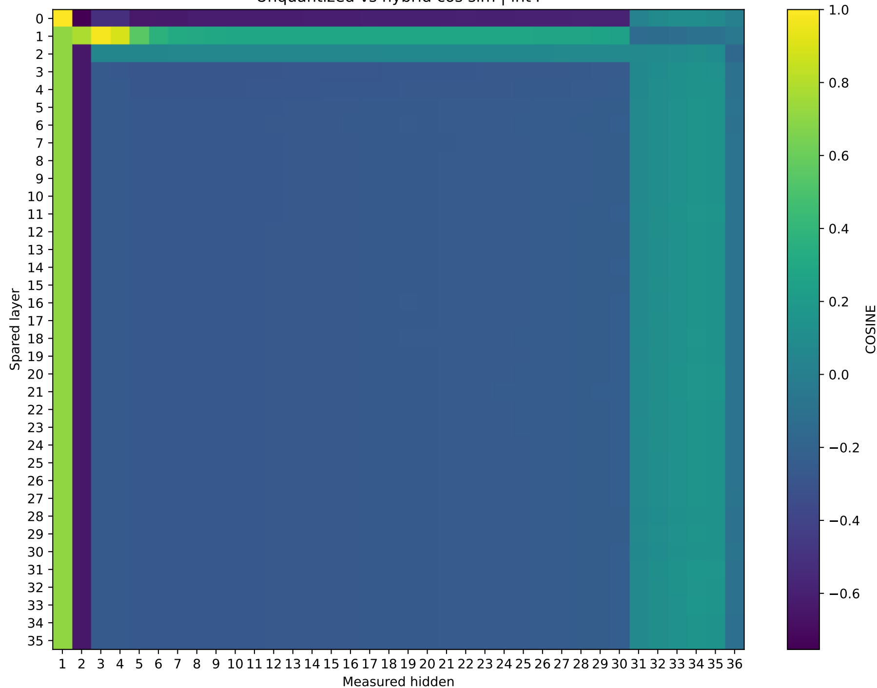
Qwen2.5-3B | Prompt 3 Unquantized vs hybrid cos sim | int4
