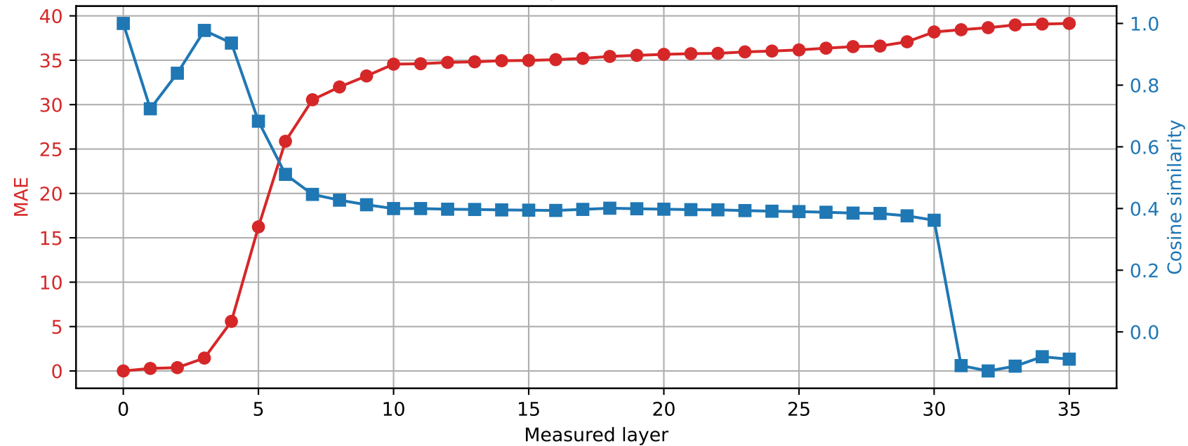
Qwen2.5-3B | Prompt 4 Spared layer 1 | Hybrid vs unquantized
