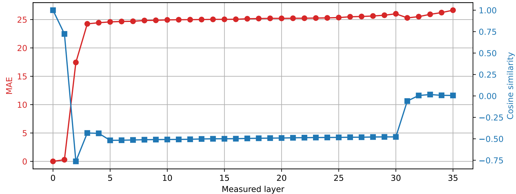
Qwen2.5-3B | Prompt 4 Spared layer 6 | Hybrid vs unquantized
