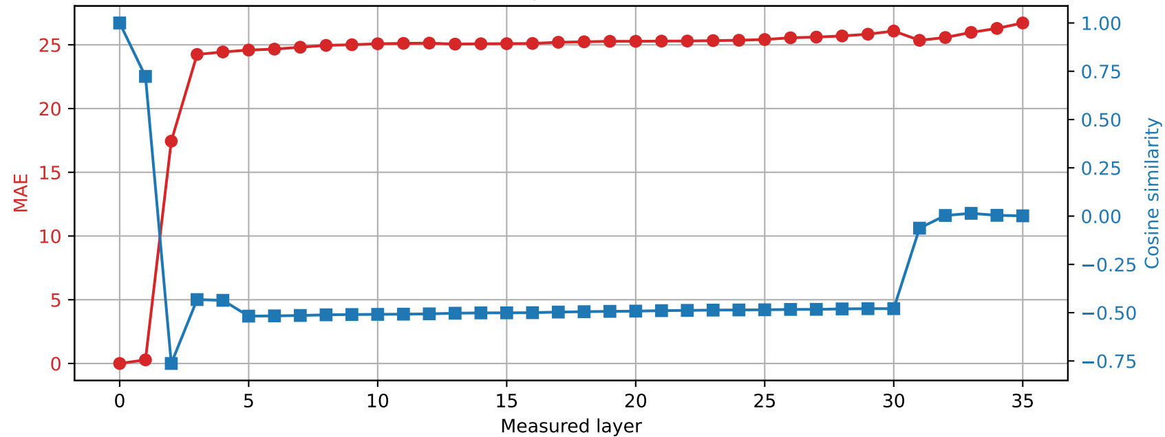
Qwen2.5-3B | Prompt 4 Spared layer 12 | Hybrid vs unquantized
