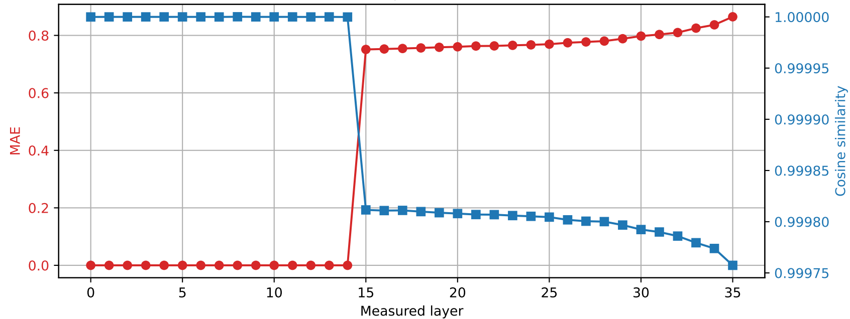
Qwen2.5-3B | Prompt 4 Spared layer 14 | Hybrid vs quantized
