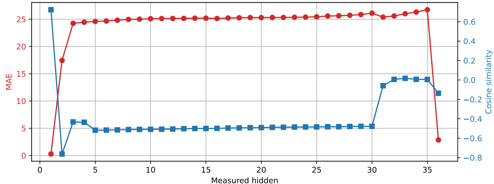
Qwen2.5-3B | Prompt 4 Spared layer 15 | Unquantized vs hybrid
