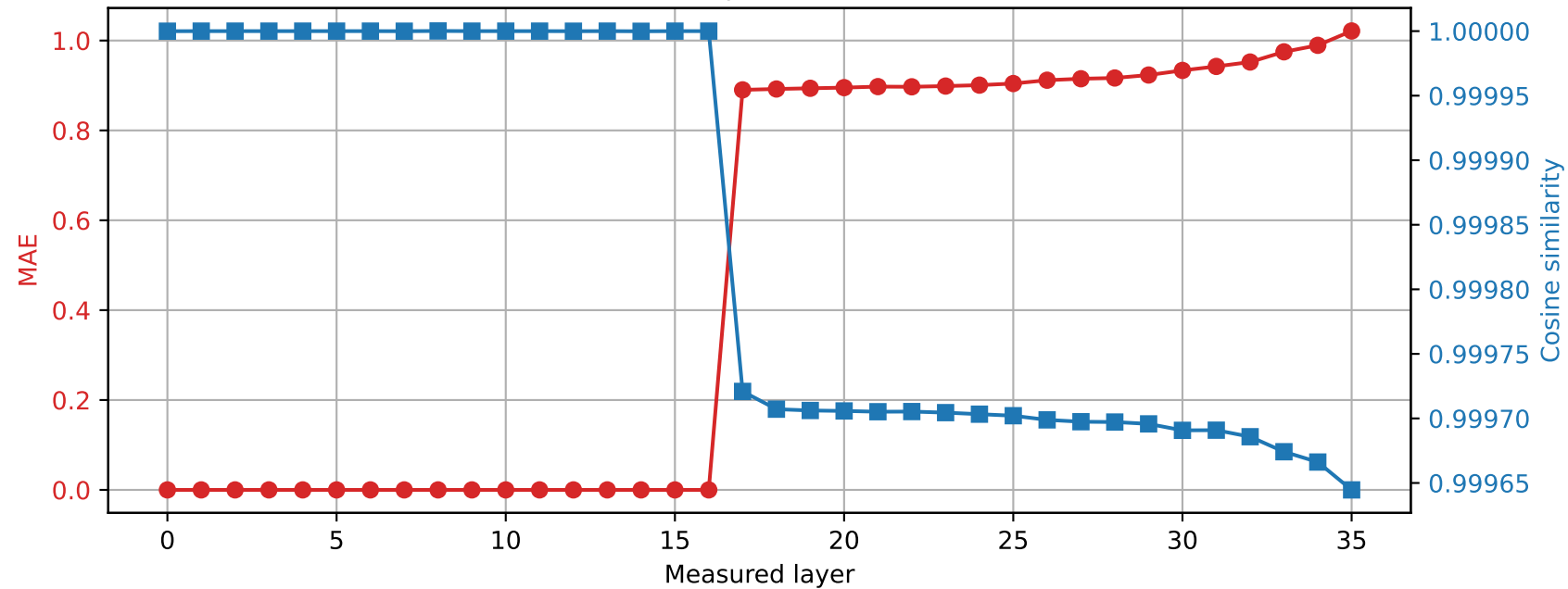
Qwen2.5-3B | Prompt 4 Spared layer 16 | Hybrid vs quantized
