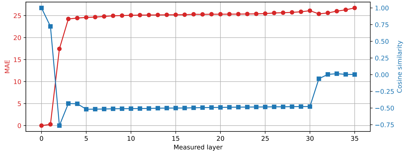
Qwen2.5-3B | Prompt 4 Spared layer 17 | Hybrid vs unquantized
