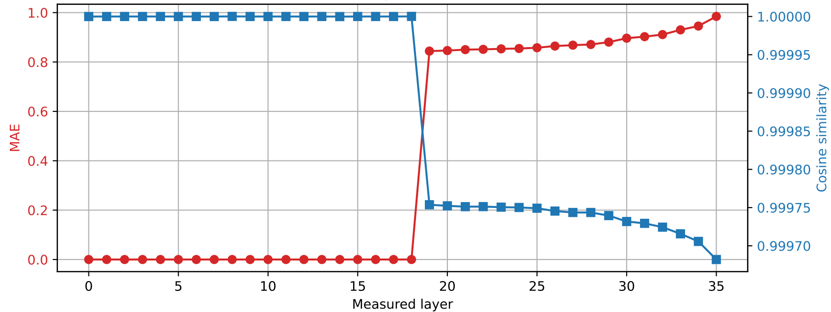
Qwen2.5-3B | Prompt 4 Spared layer 18 | Hybrid vs quantized
