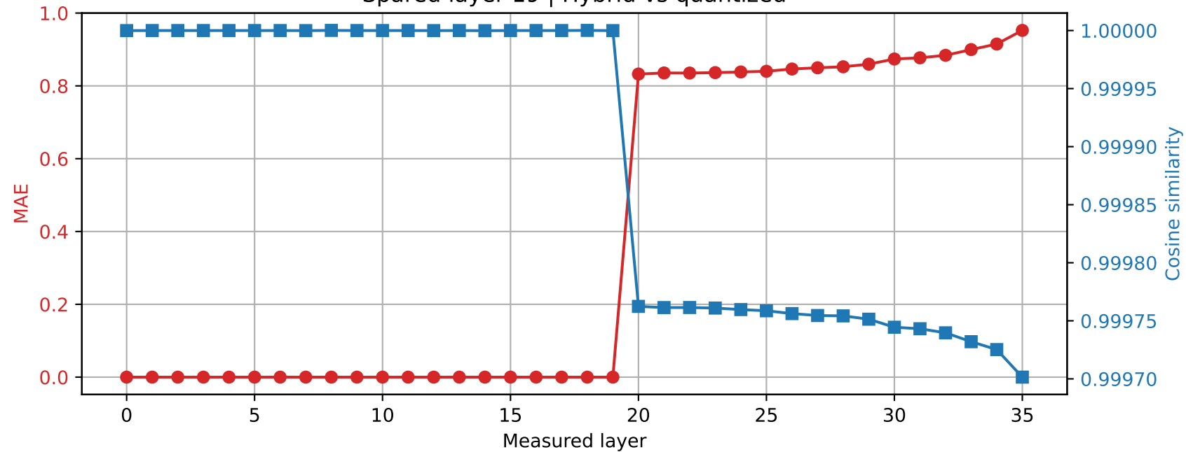
Qwen2.5-3B | Prompt 4 Spared layer 19 | Hybrid vs quantized
