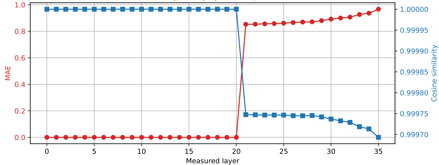
Qwen2.5-3B | Prompt 4 Spared layer 20 | Hybrid vs quantized
