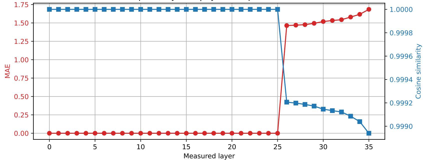
Qwen2.5-3B | Prompt 4 Spared layer 25 | Hybrid vs quantized
