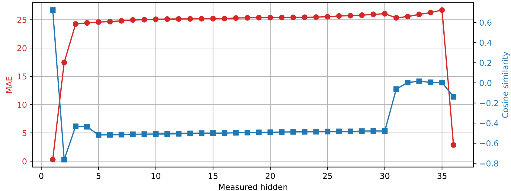
Qwen2.5-3B | Prompt 4 Spared layer 29 | Unquantized vs hybrid
