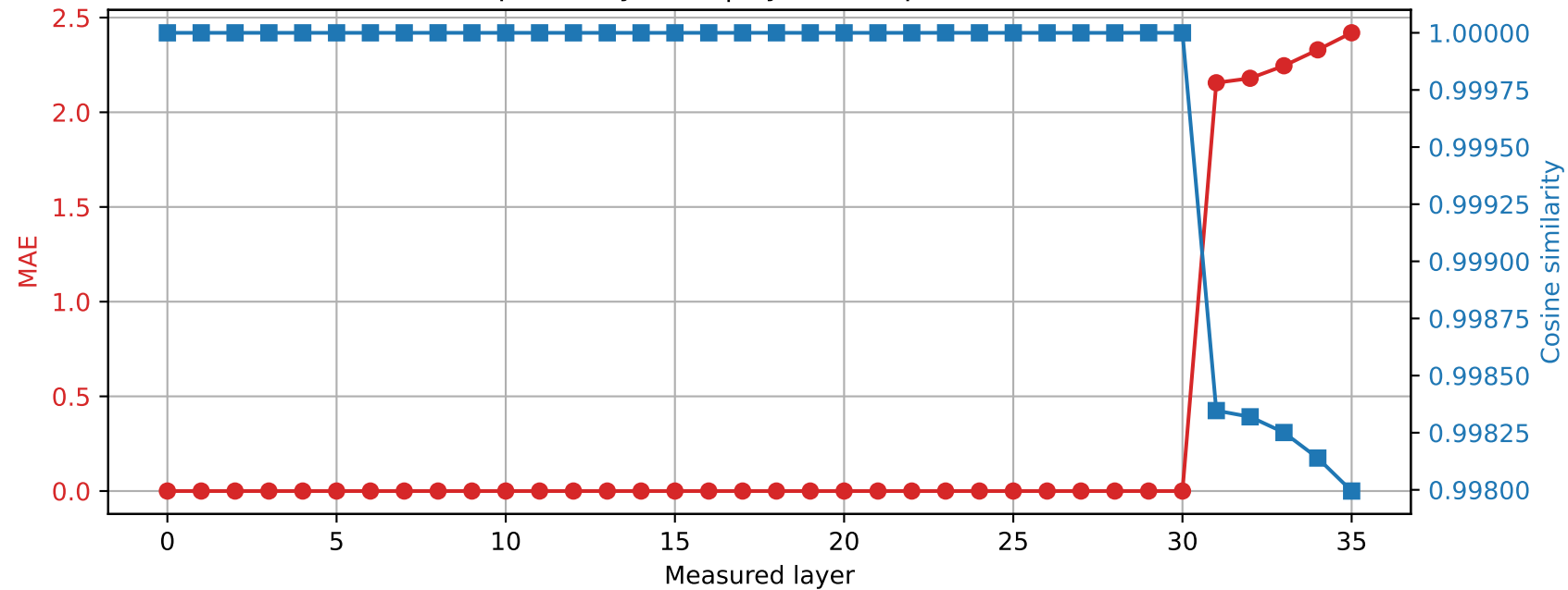
Qwen2.5-3B | Prompt 4 Spared layer 30 | Hybrid vs quantized
