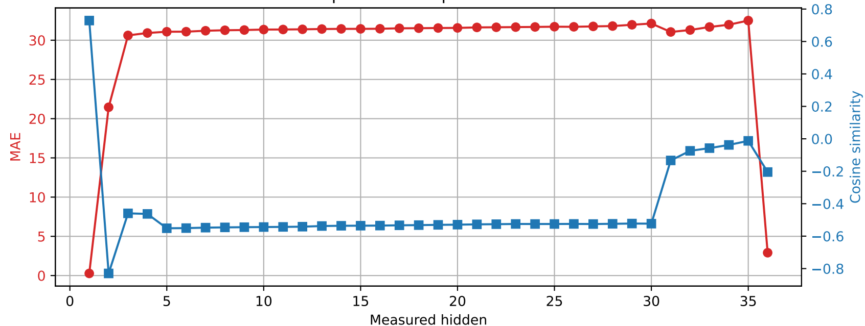
Qwen2.5-3B | Prompt 0 Unquantized vs quantized int4
