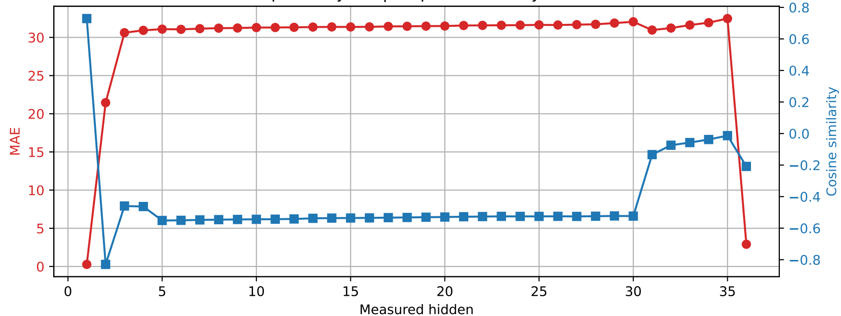
Qwen2.5-3B | Prompt 0 Spared layer 5 | Unquantized vs hybrid
