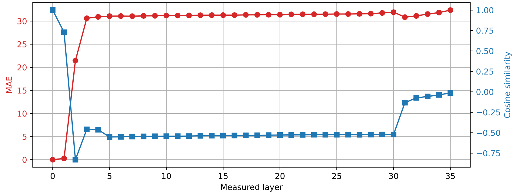
Qwen2.5-3B | Prompt 0 Spared layer 6 | Hybrid vs unquantized
