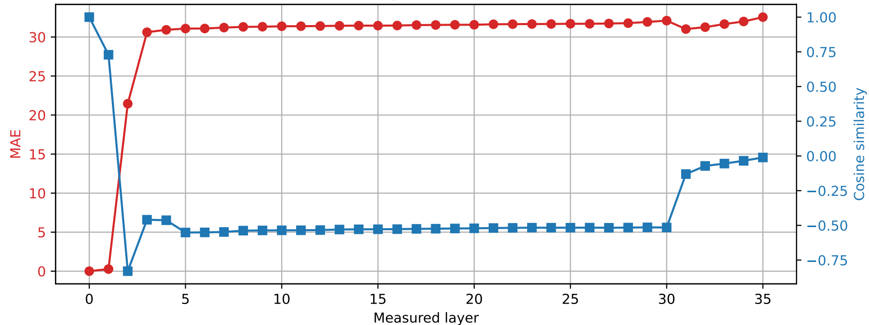
Qwen2.5-3B | Prompt 0 Spared layer 7 | Hybrid vs unquantized
