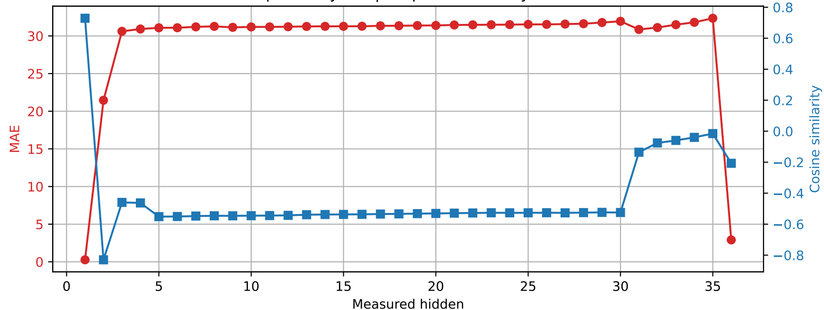
Qwen2.5-3B | Prompt 0 Spared layer 8 | Unquantized vs hybrid
