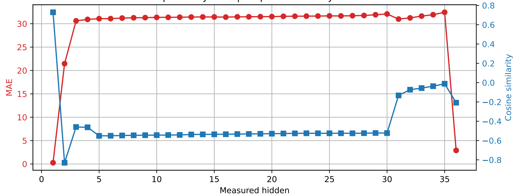
Qwen2.5-3B | Prompt 0 Spared layer 15 | Unquantized vs hybrid
