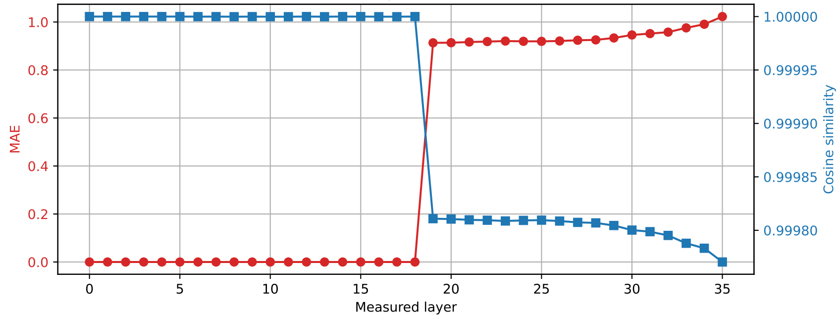
Qwen2.5-3B | Prompt 0 Spared layer 18 | Hybrid vs quantized
