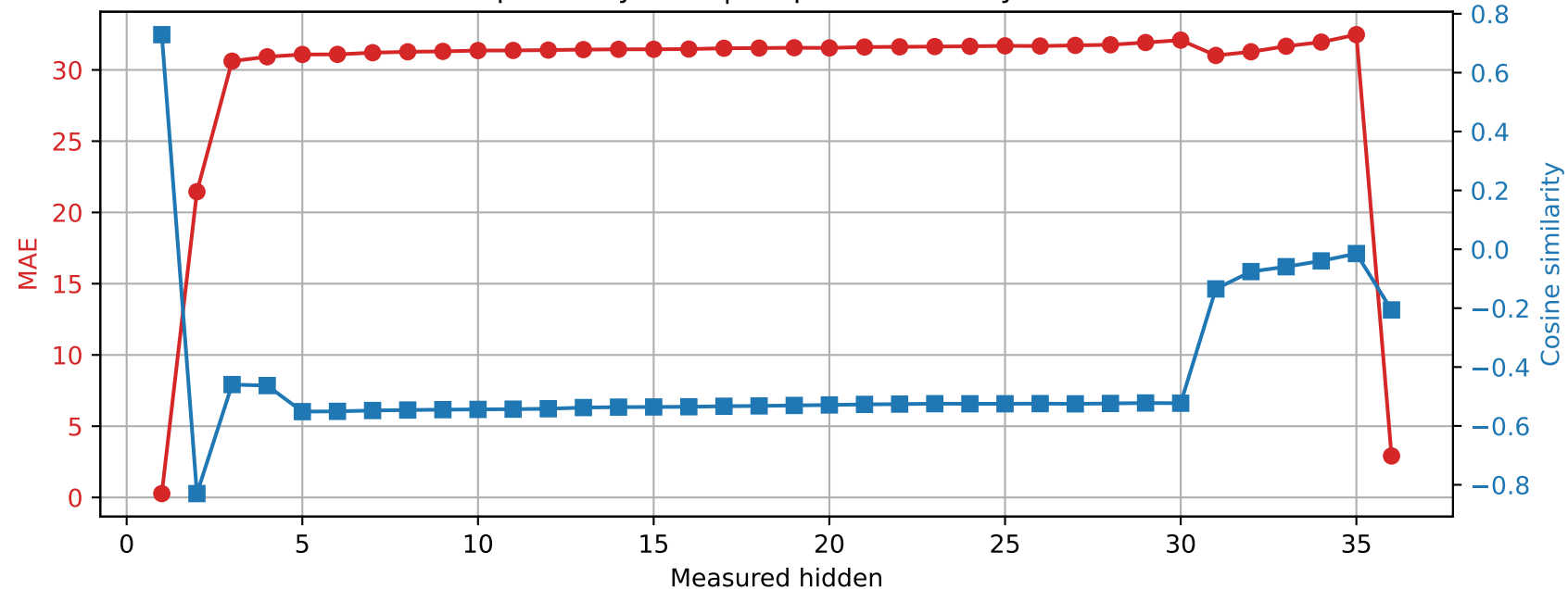
Qwen2.5-3B | Prompt 0 Spared layer 19 | Unquantized vs hybrid
