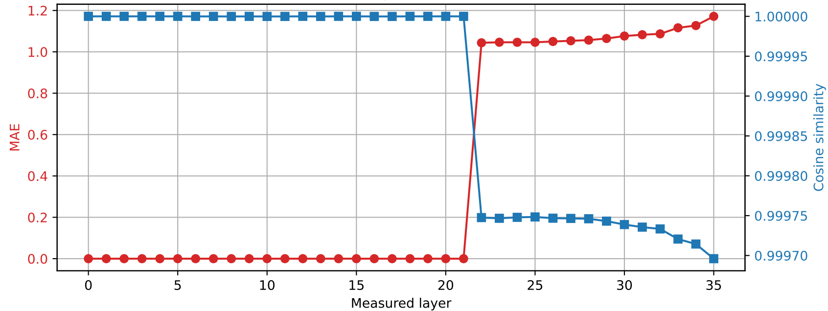
Qwen2.5-3B | Prompt 0 Spared layer 21 | Hybrid vs quantized
