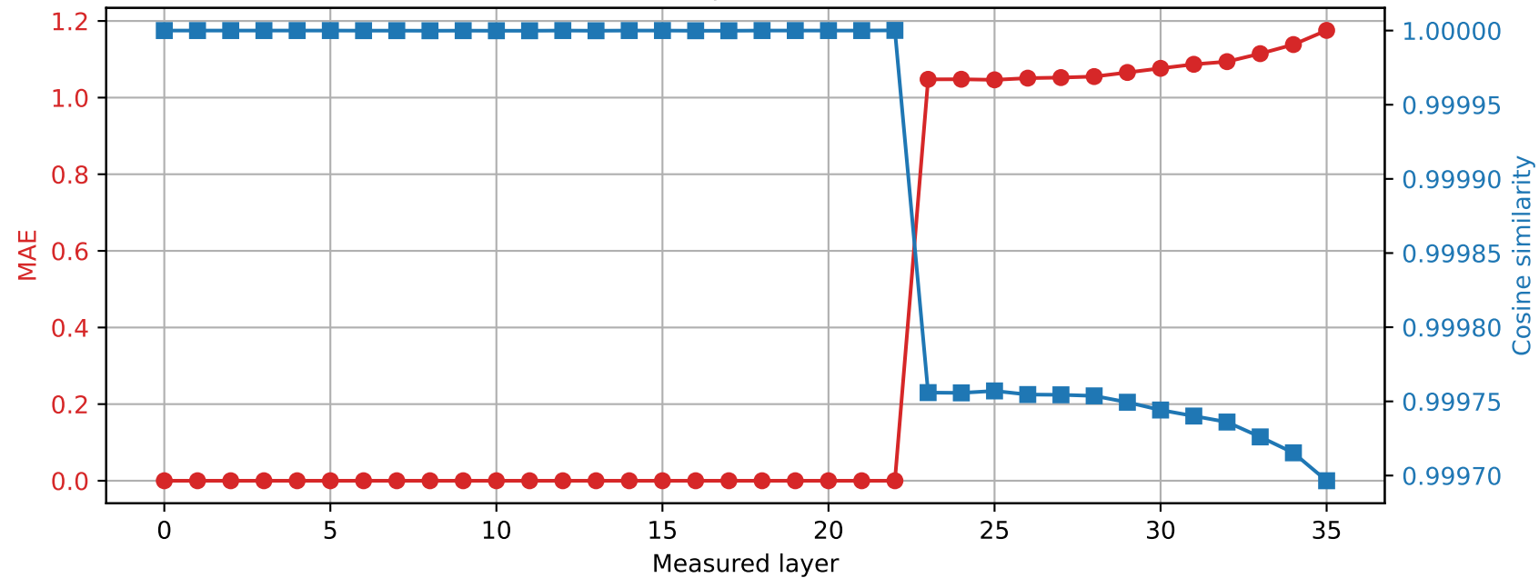
Qwen2.5-3B | Prompt 0 Spared layer 22 | Hybrid vs quantized
