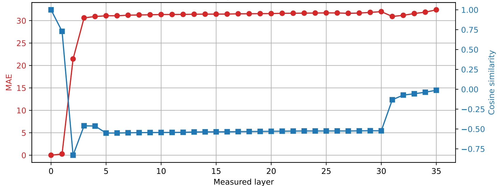
Qwen2.5-3B | Prompt 0 Spared layer 26 | Hybrid vs unquantized
