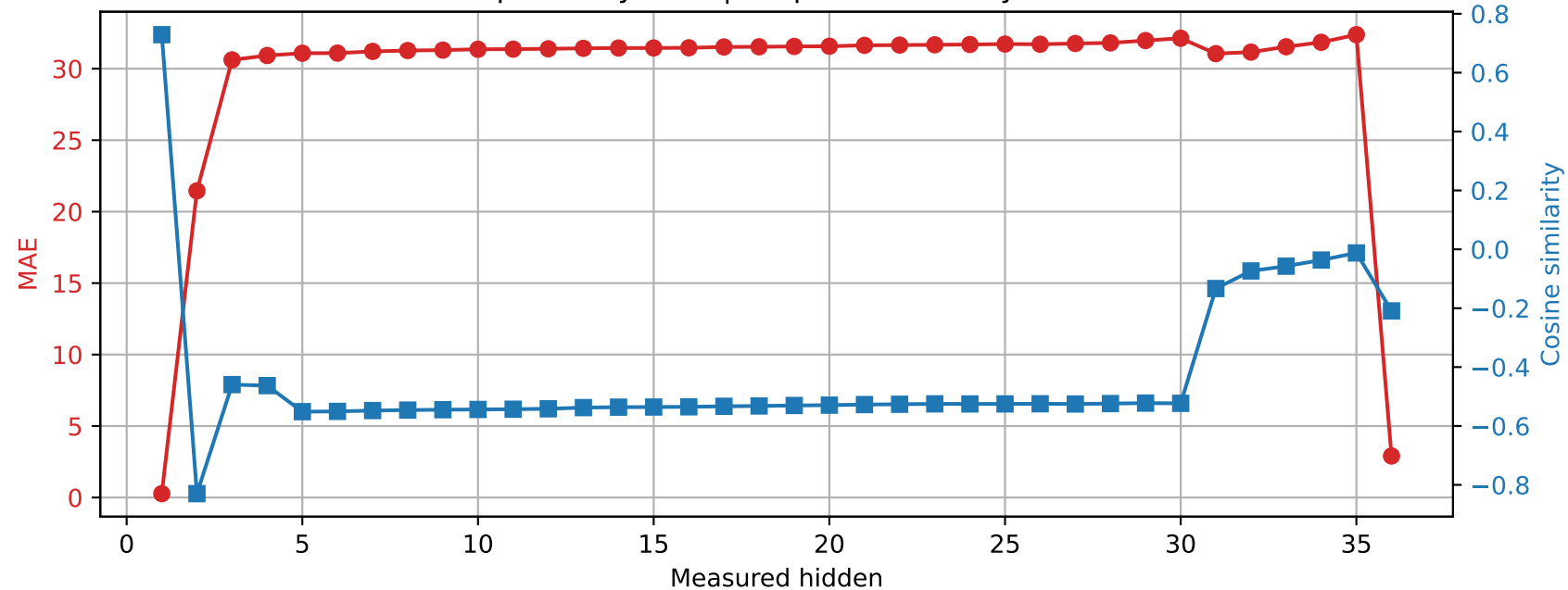
Qwen2.5-3B | Prompt 0 Spared layer 31 | Unquantized vs hybrid
