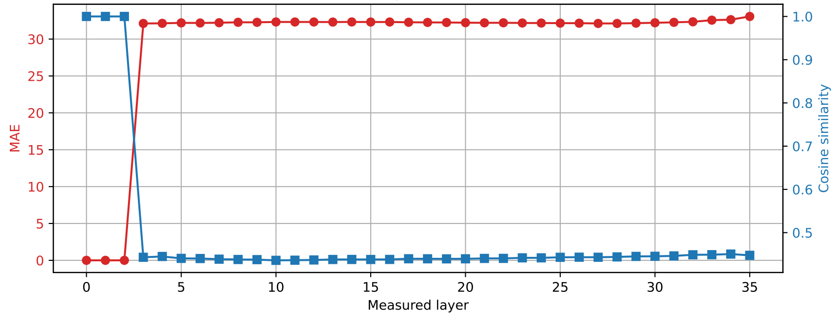
Qwen2.5-3B | Prompt 1 Spared layer 2 | Hybrid vs quantized
