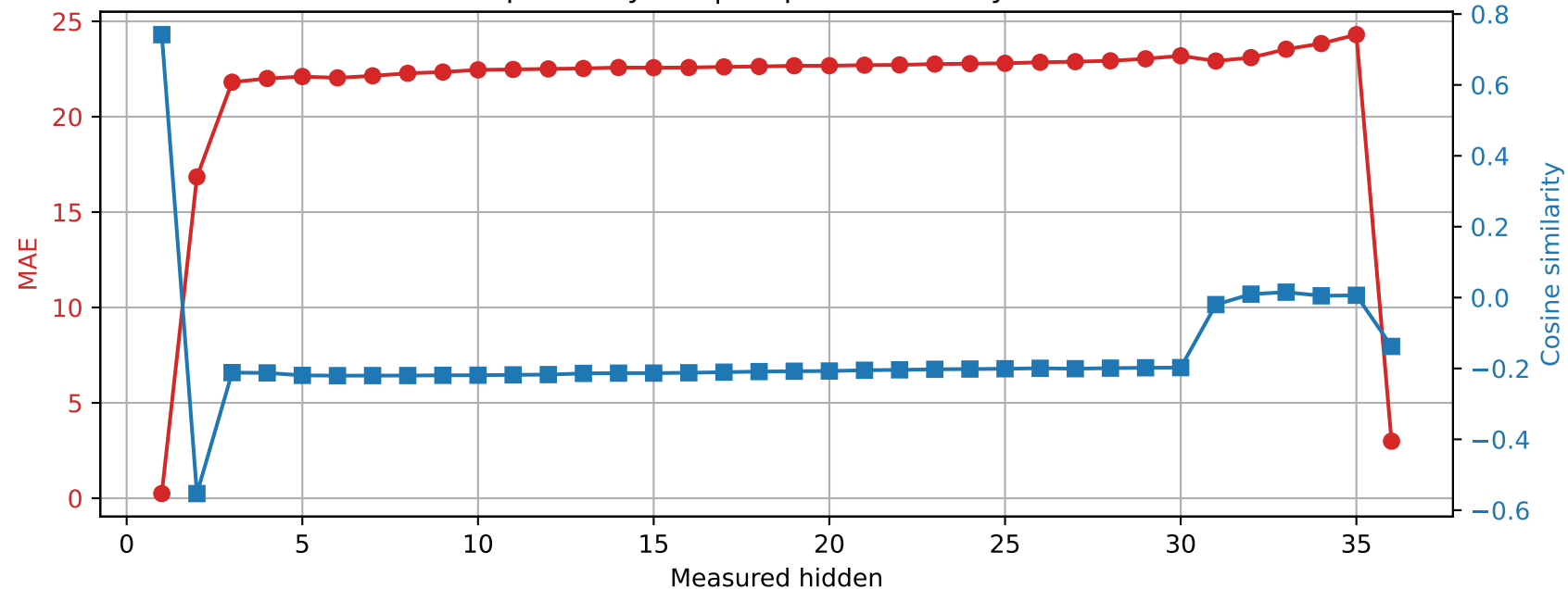
Qwen2.5-3B | Prompt 1 Spared layer 5 | Unquantized vs hybrid
