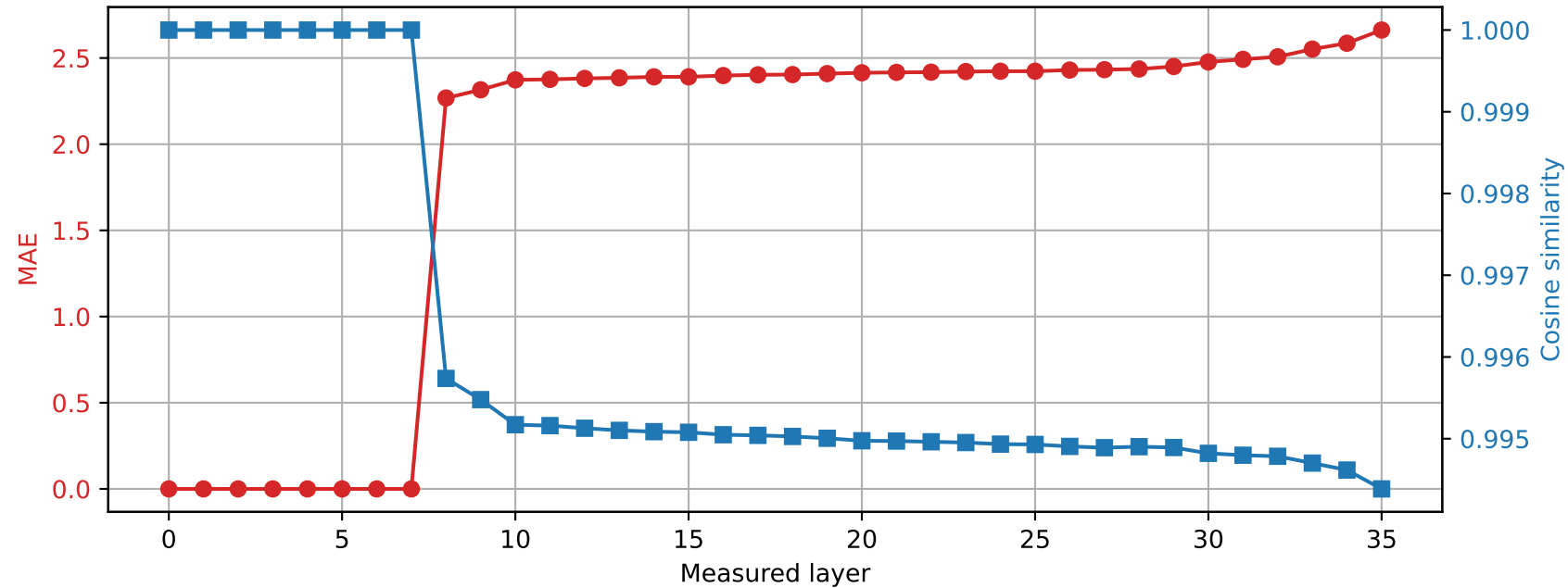
Qwen2.5-3B | Prompt 1 Spared layer 7 | Hybrid vs quantized
