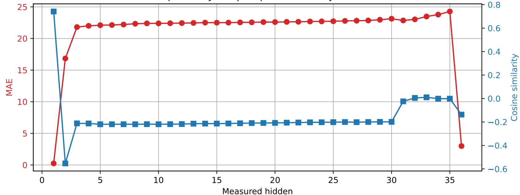
Qwen2.5-3B | Prompt 1 Spared layer 9 | Unquantized vs hybrid
