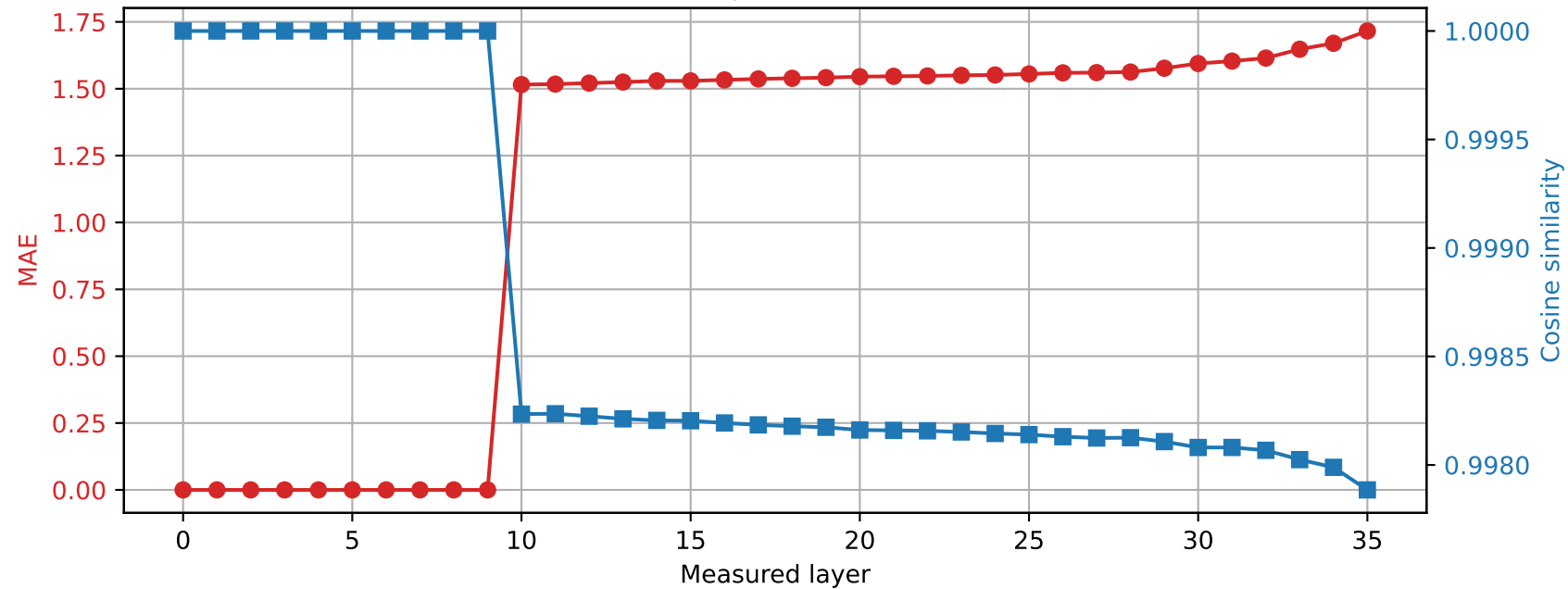
Qwen2.5-3B | Prompt 1 Spared layer 9 | Hybrid vs quantized
