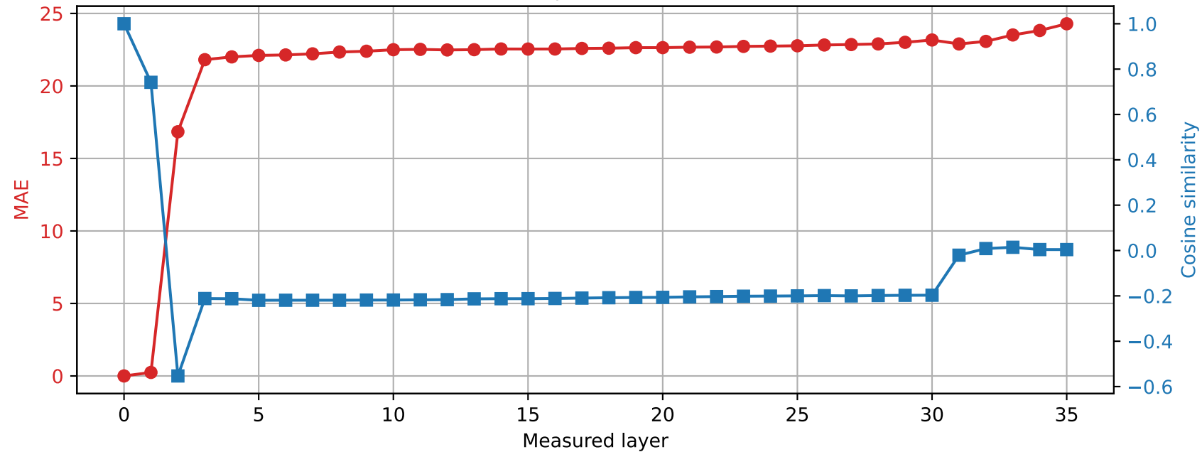
Qwen2.5-3B | Prompt 1 Spared layer 11 | Hybrid vs unquantized
