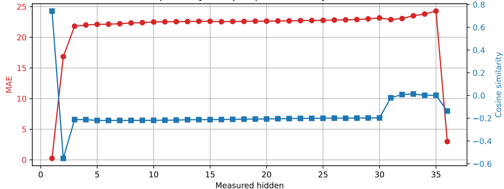
Qwen2.5-3B | Prompt 1 Spared layer 15 | Unquantized vs hybrid
