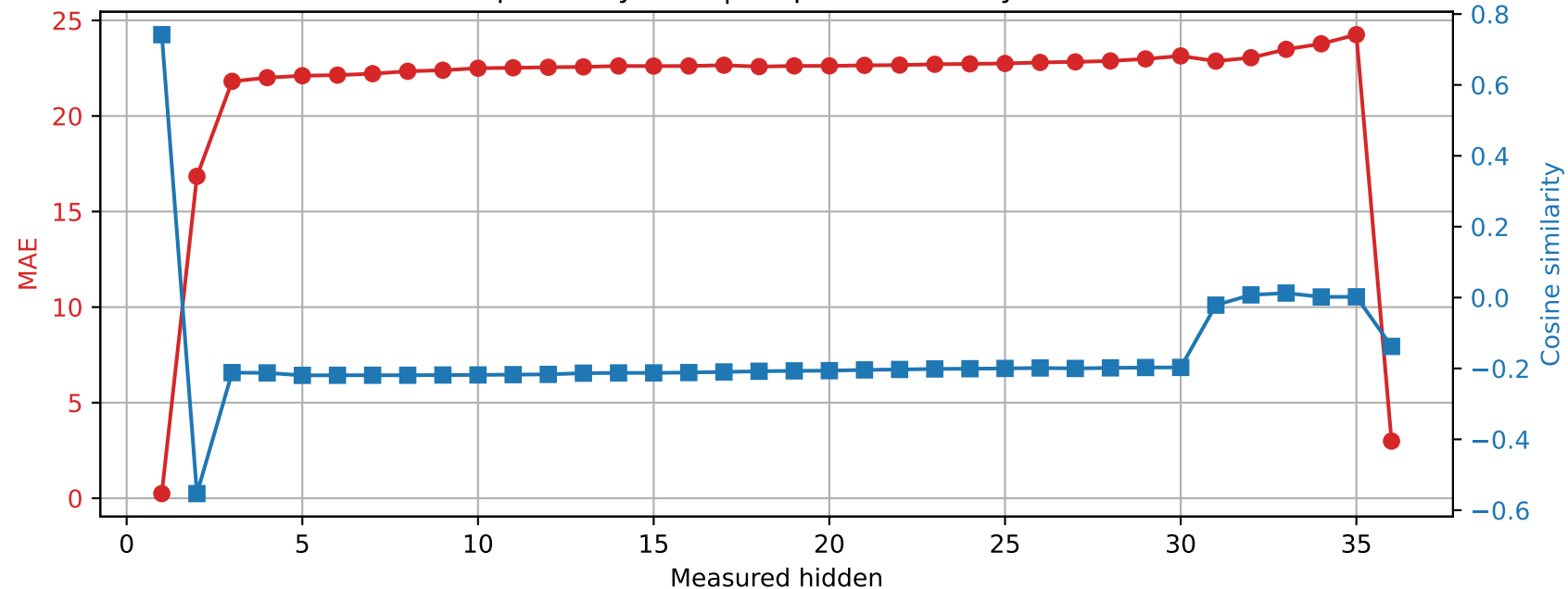
Qwen2.5-3B | Prompt 1 Spared layer 17 | Unquantized vs hybrid
