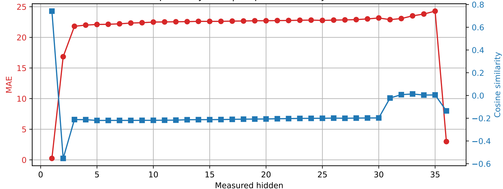
Qwen2.5-3B | Prompt 1 Spared layer 24 | Unquantized vs hybrid
