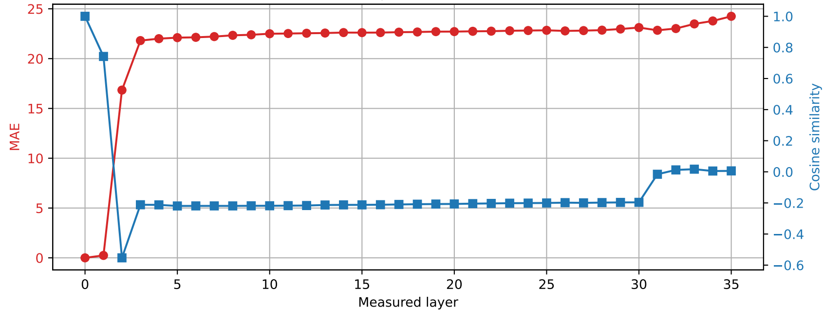
Qwen2.5-3B | Prompt 1 Spared layer 25 | Hybrid vs unquantized
