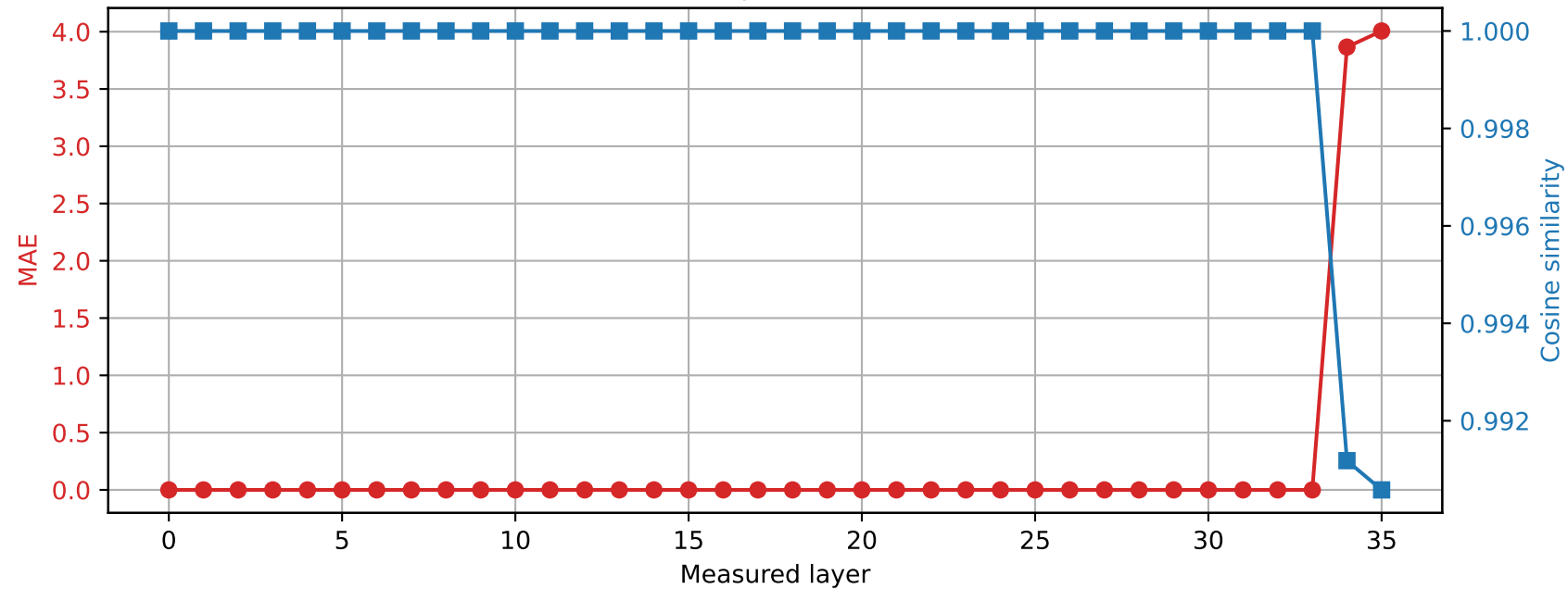
Qwen2.5-3B | Prompt 1 Spared layer 33 | Hybrid vs quantized
