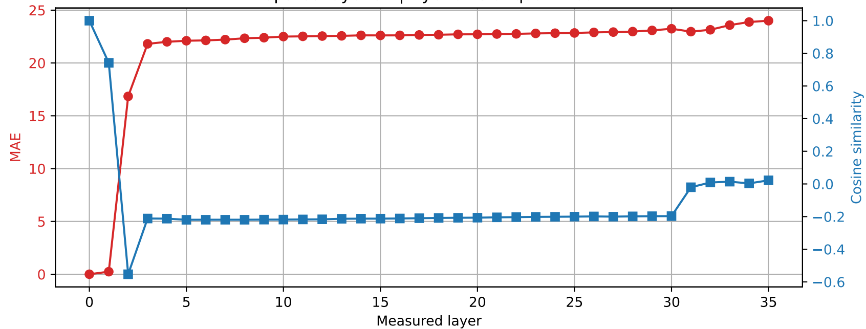
Qwen2.5-3B | Prompt 1 Spared layer 34 | Hybrid vs unquantized
