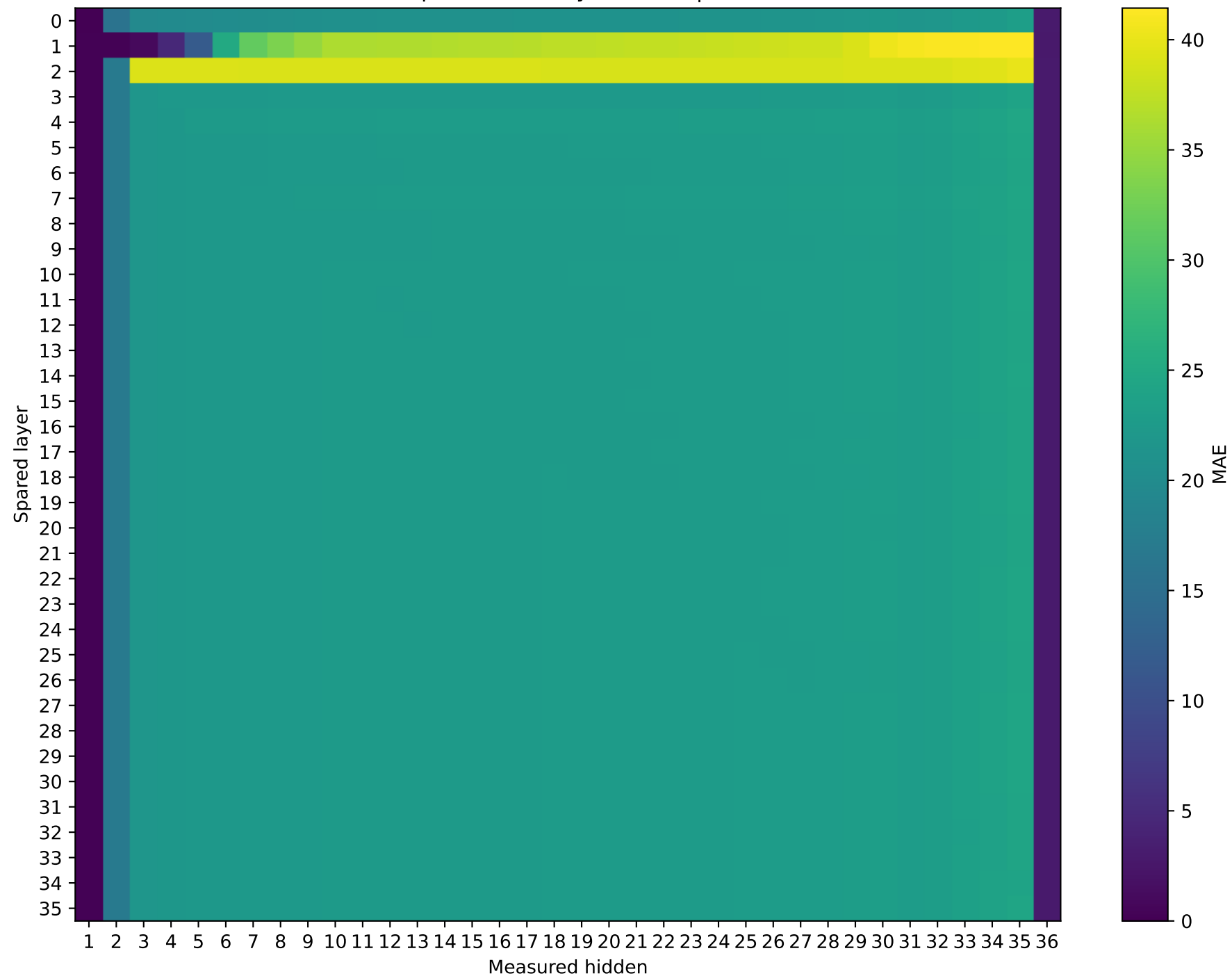
Qwen2.5-3B | Prompt 1 Unquantized vs hybrid MAE | int4
