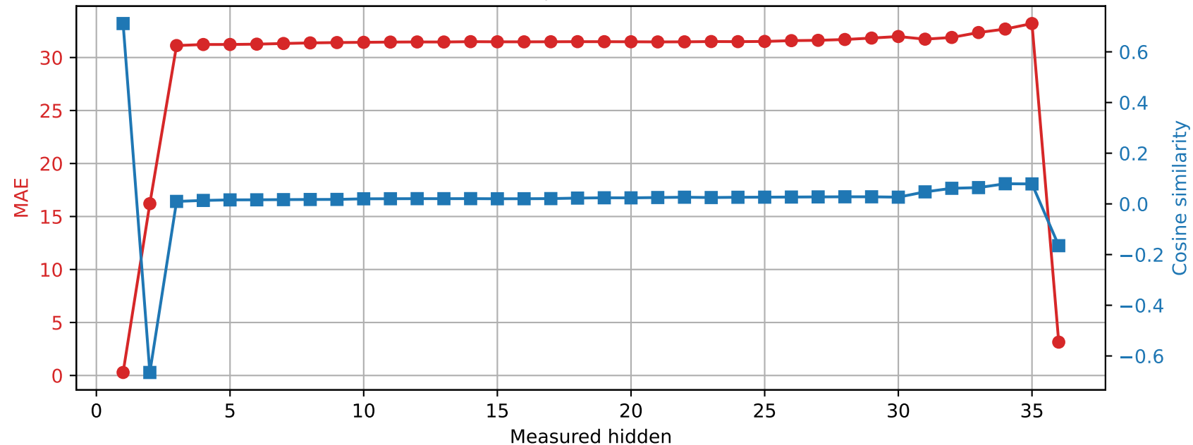
Qwen2.5-3B | Prompt 2 Spared layer 2 | Unquantized vs hybrid
