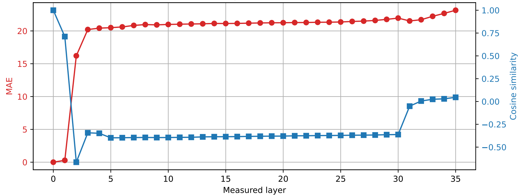
Qwen2.5-3B | Prompt 2 Spared layer 8 | Hybrid vs unquantized
