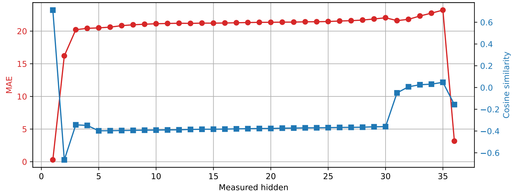
Qwen2.5-3B | Prompt 2 Spared layer 12 | Unquantized vs hybrid
