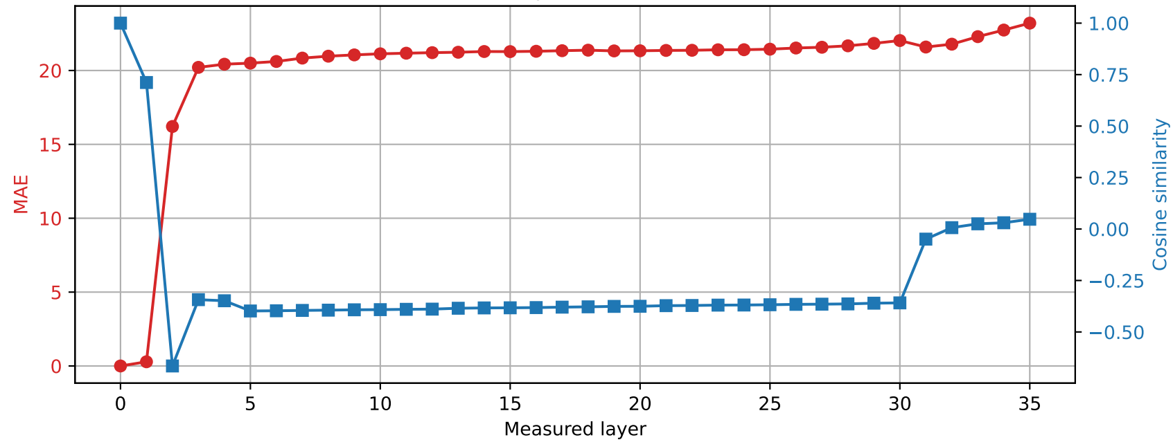
Qwen2.5-3B | Prompt 2 Spared layer 18 | Hybrid vs unquantized
